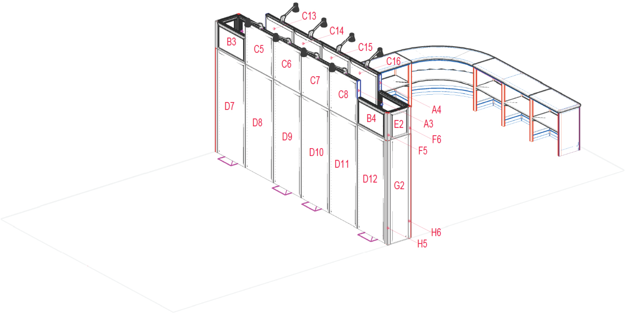
REAR PERSPECTIVE
